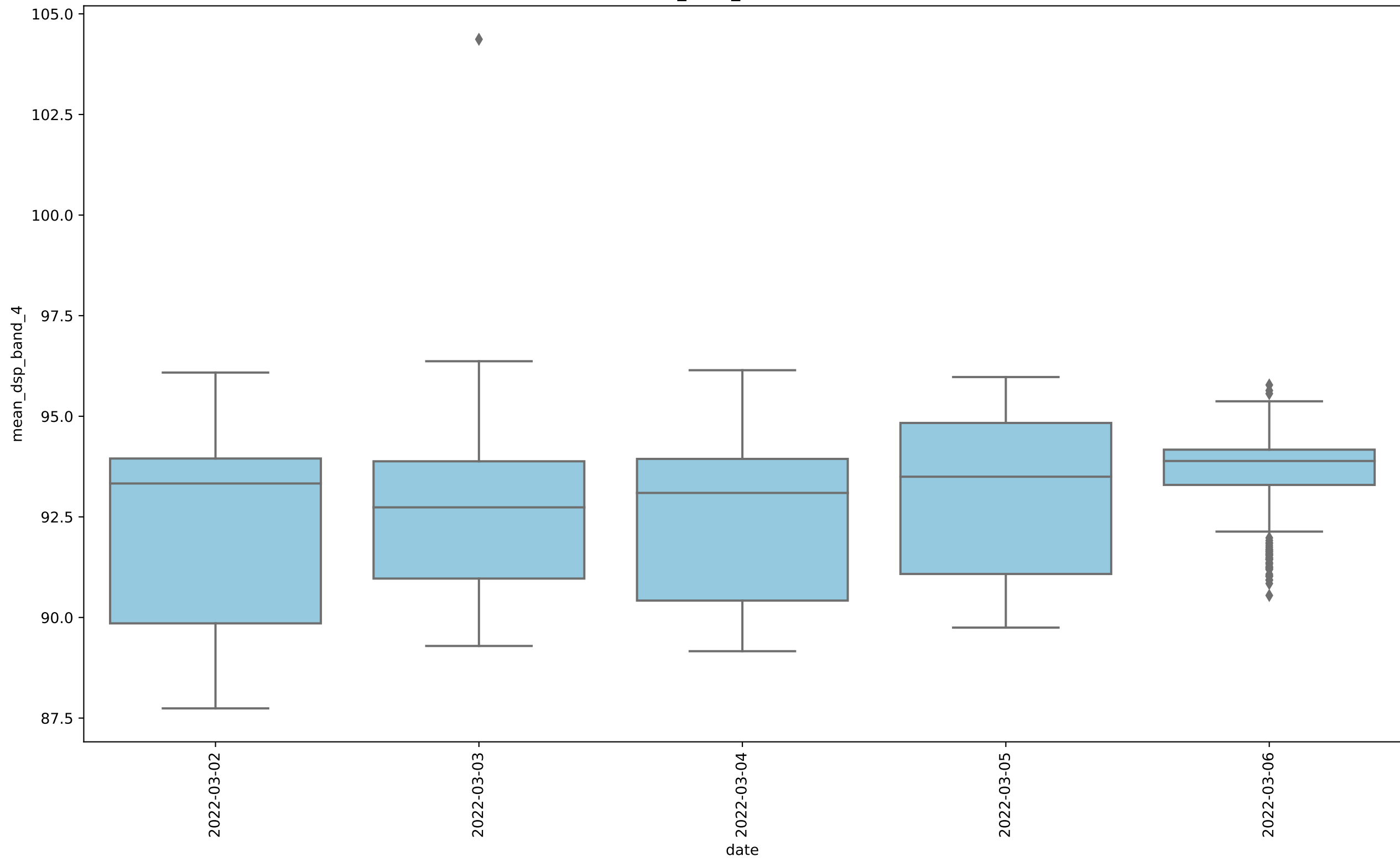
RAYOL_2022_mean, band 4
