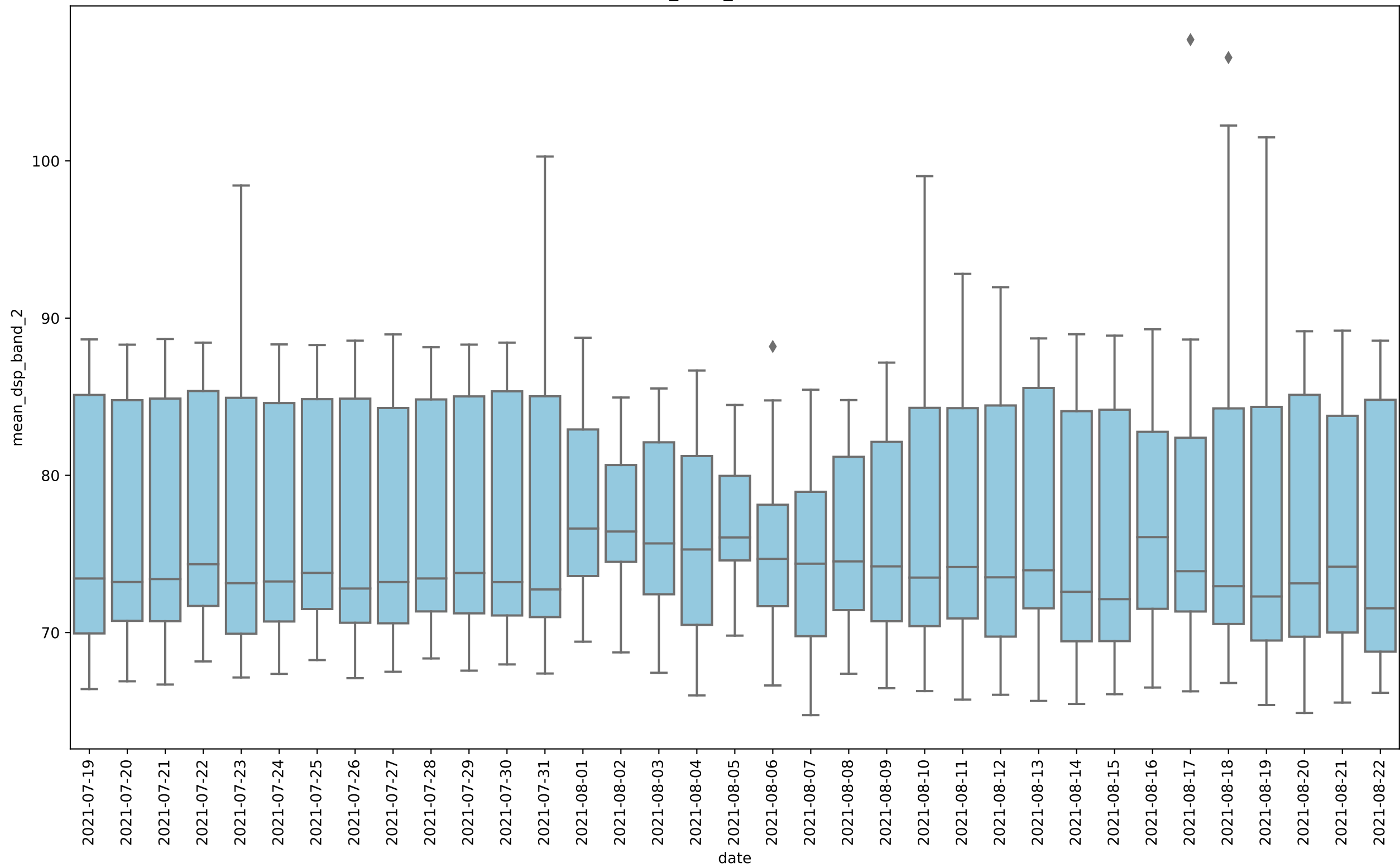
RAYOL_2021_mean, band 2
