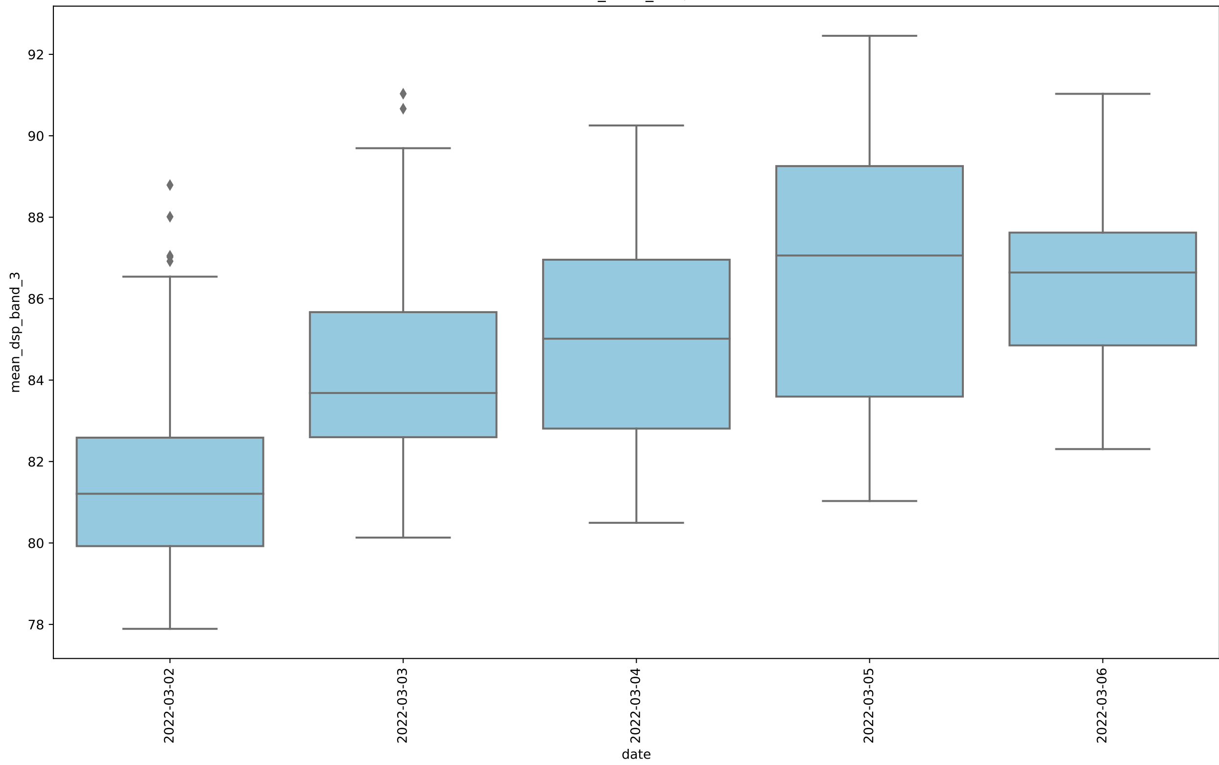
RASCASS_2022_min, band 3
