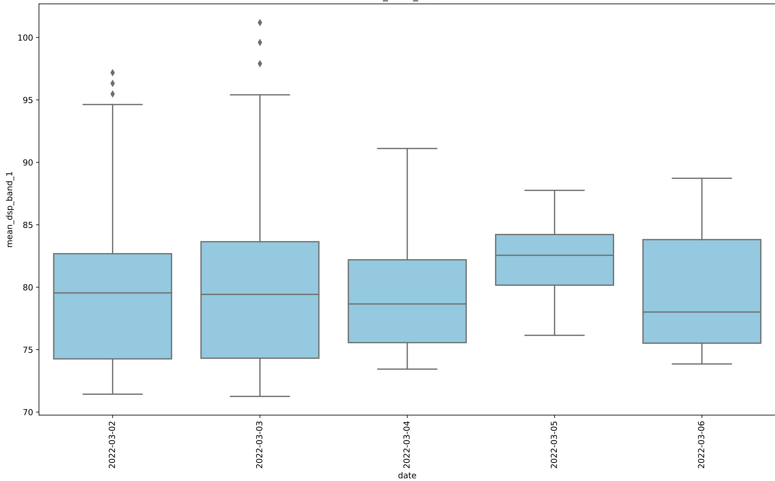
RASCASS_2022_min, band 1
