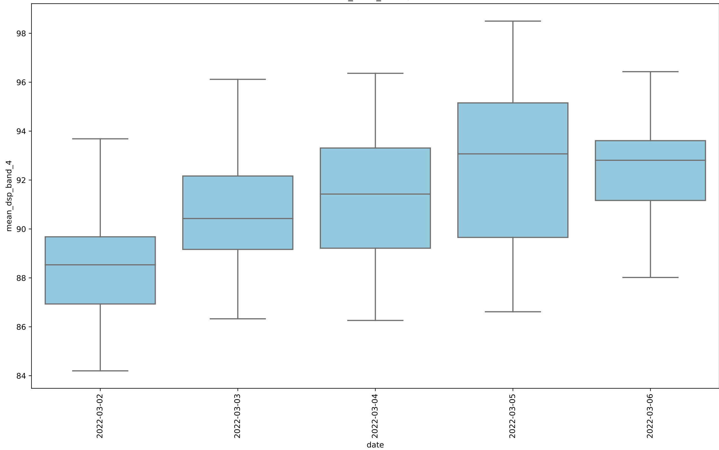
RASCASS_2022_mean, band 4
