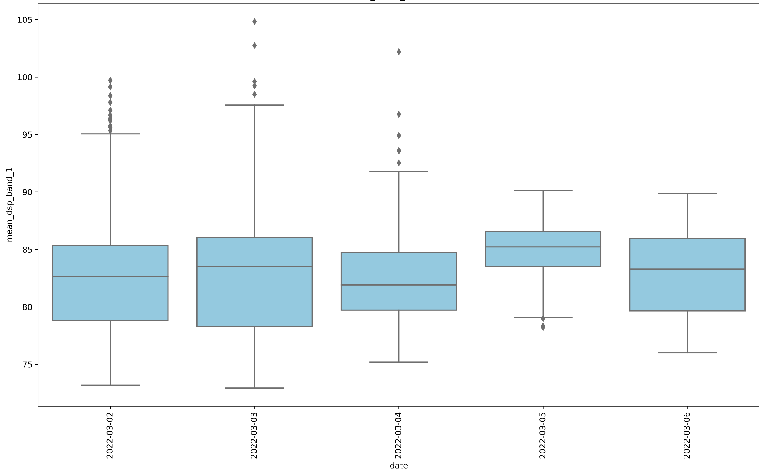
RASCASS_2022_mean, band 1
