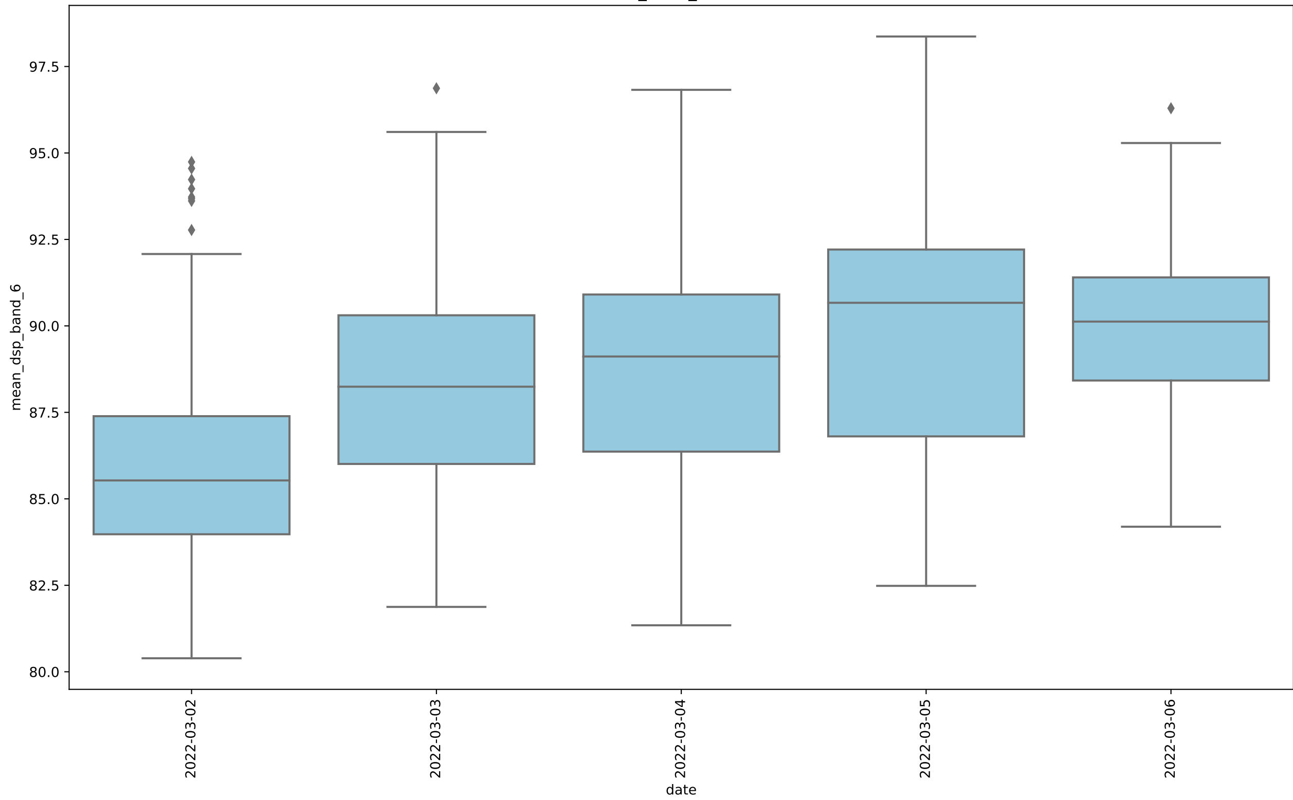
RASCASS_2022_max, band 6
