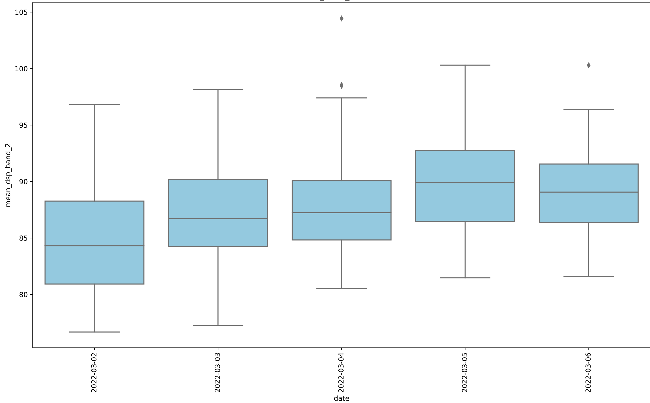
RASCASS_2022_max, band 2
