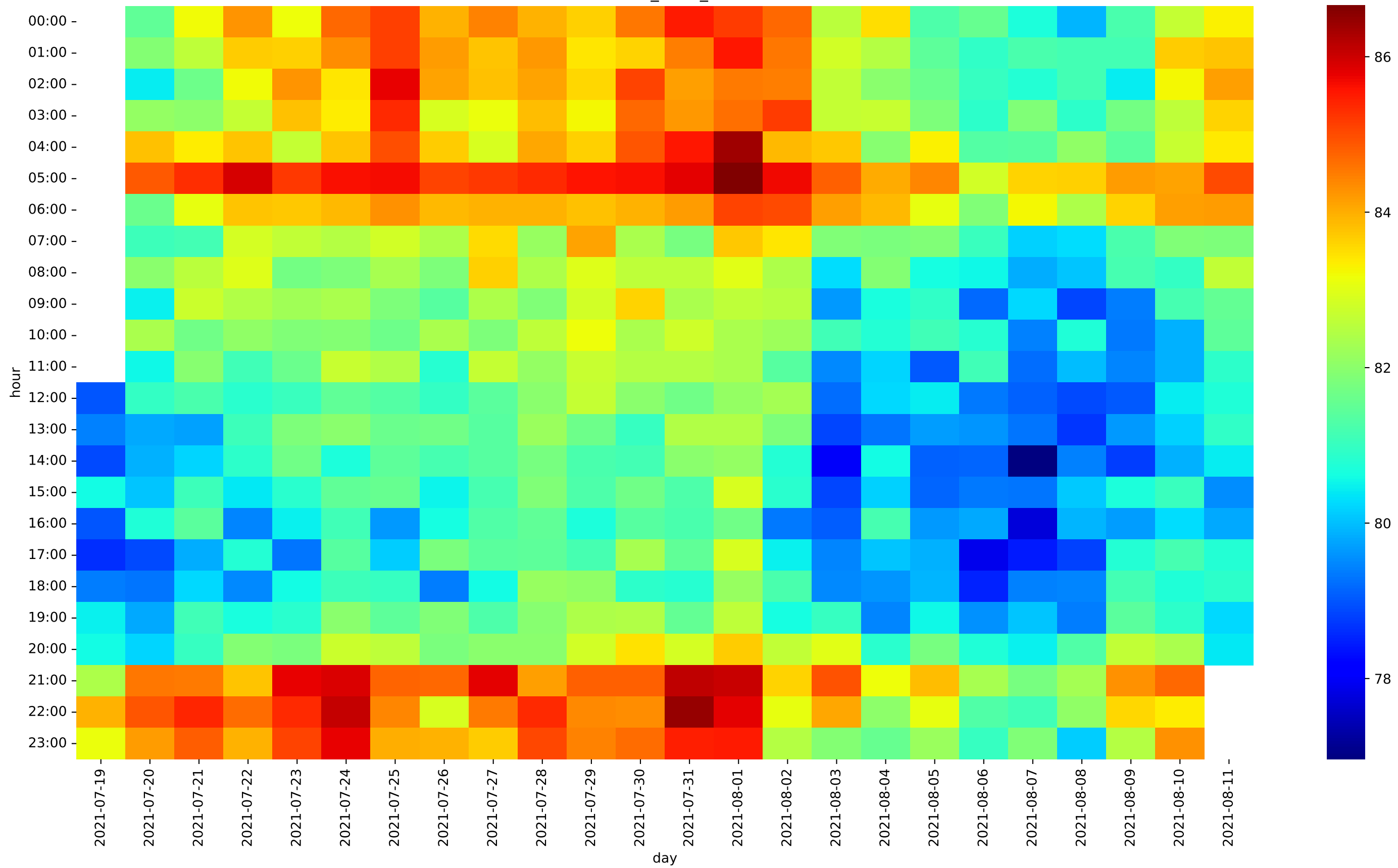
RASCASS_2021_mean
