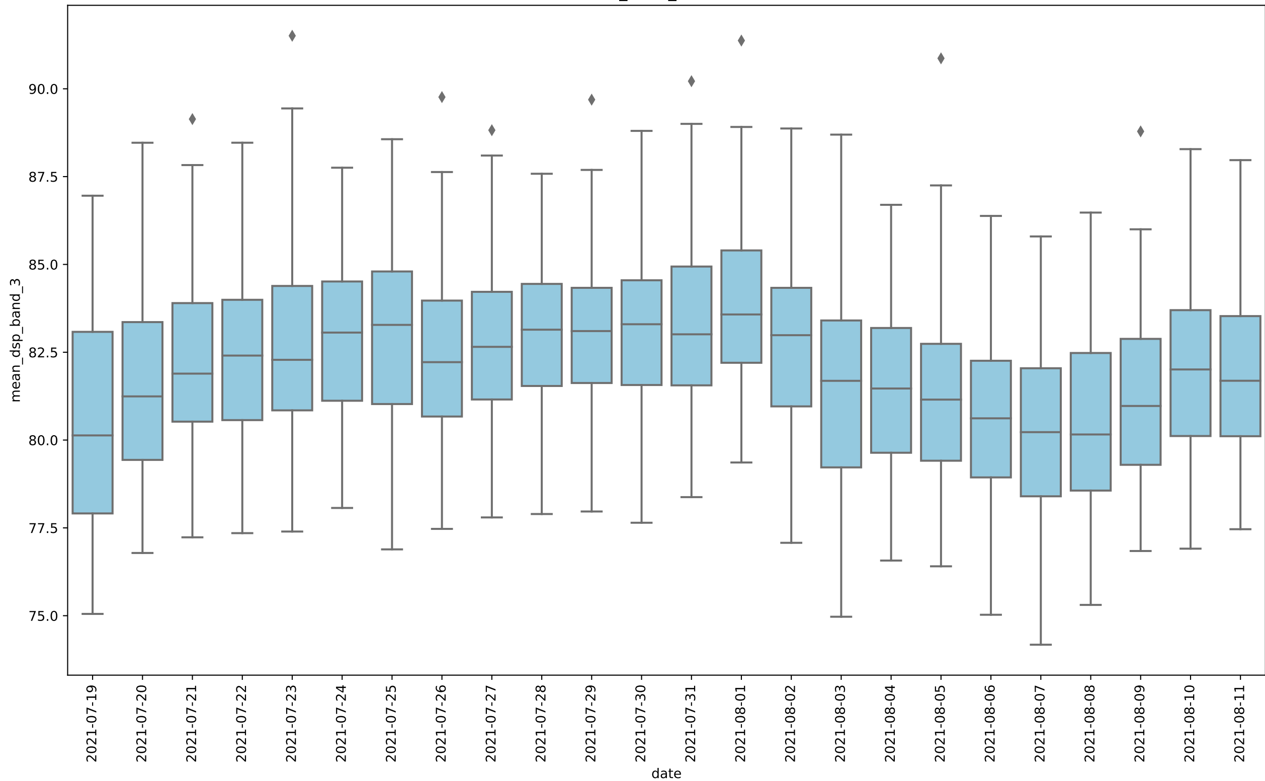
RASCASS_2021_mean, band 3
