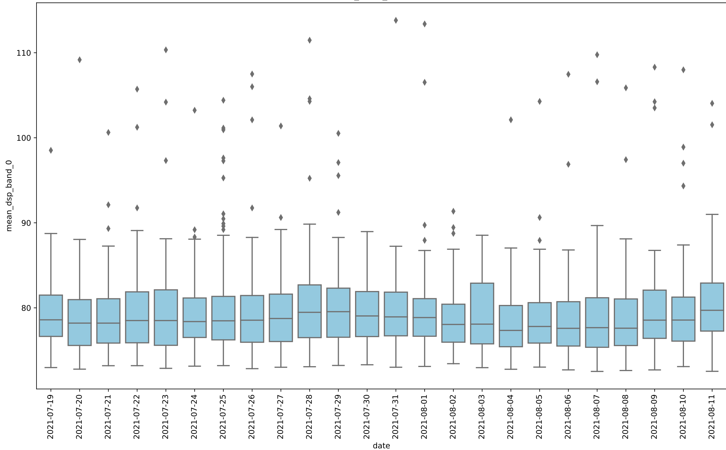
RASCASS_2021_mean, band 0
