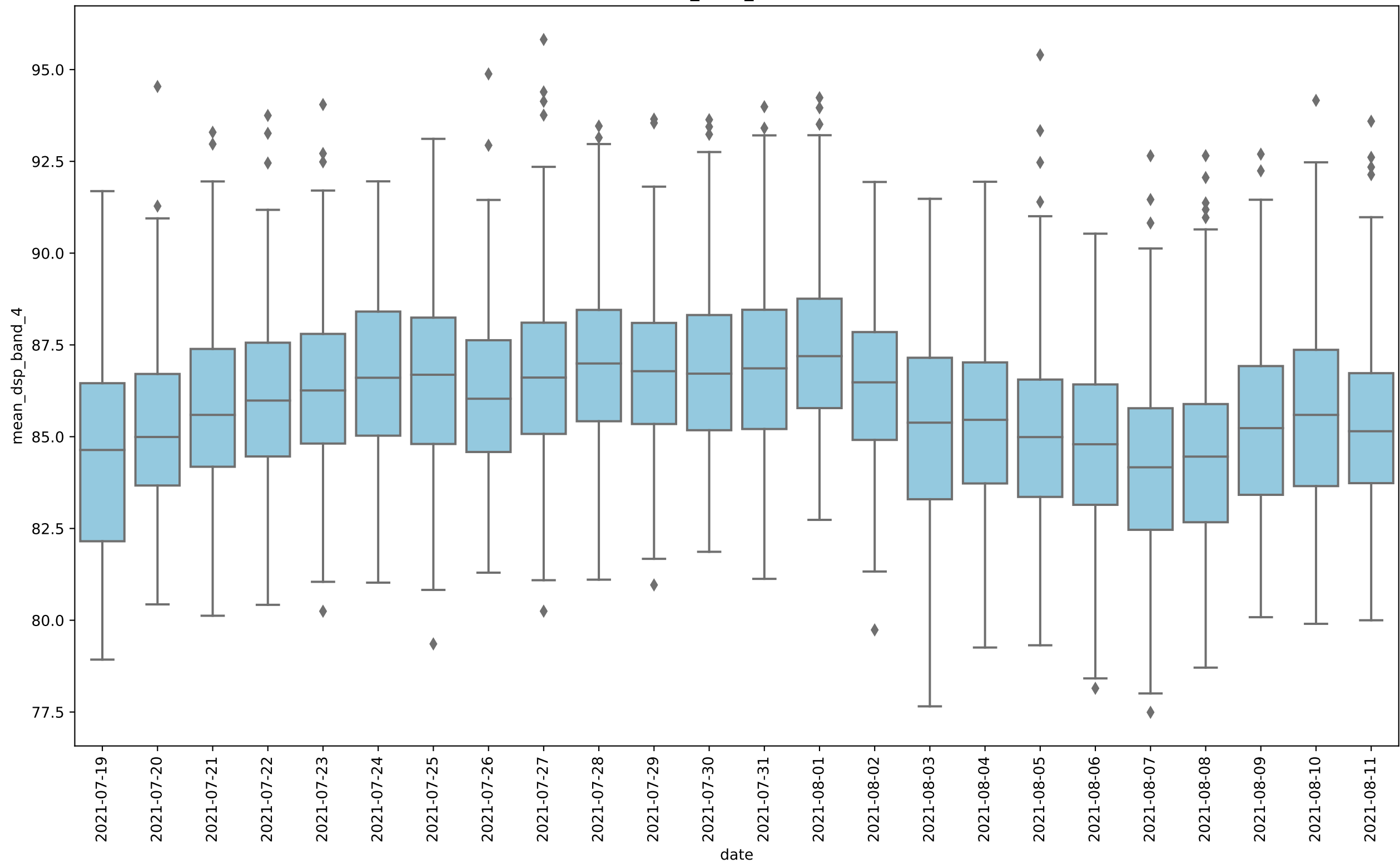
RASCASS_2021_max, band 4
