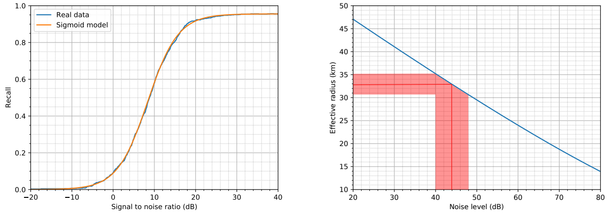
Figure 7. Left: Recall of the CNN and the sigmoid model of this recall curve. Right: Effective radius of the antenna for varying background noise level. The red line (zone) corresponds to the average (standard deviation) noise level at 12.8 kHz in the area.
