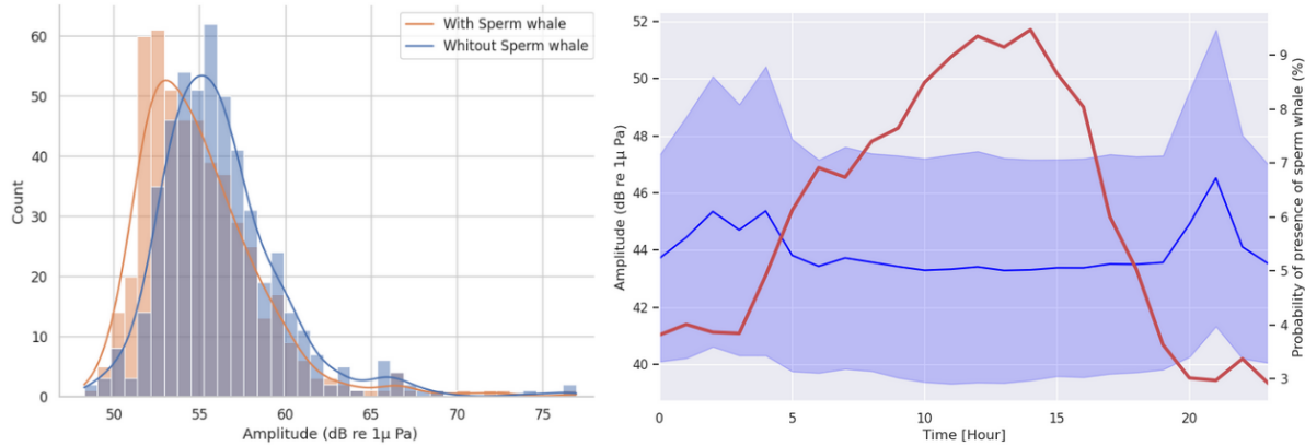
Figure 3. Left: Distribution of the amplitude for the octave 12800 Hz according to presence/absence of sperm whales. Right: Superposition of dial pattern of amplitudes for the octave 12800 Hz and probability of presence of sperm whales.
