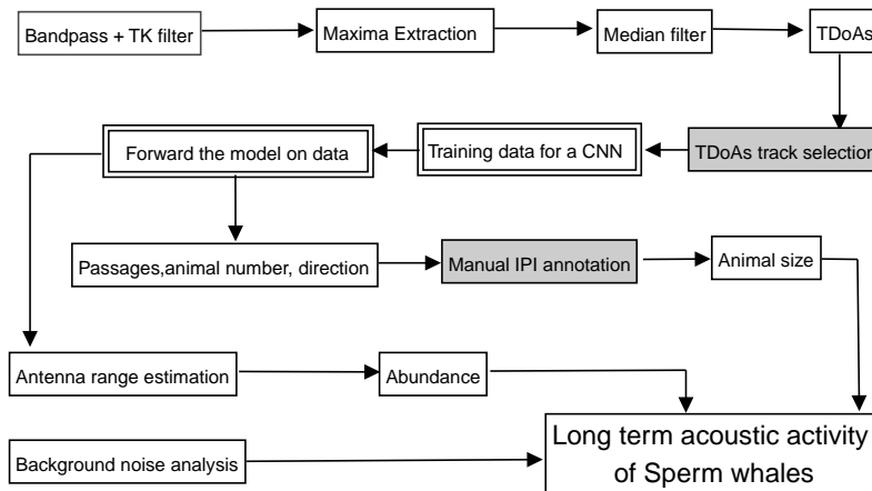
Figure 6. Summary diagram of the analysis. Gray boxes: semi-manual process. Double line: Deep learning process.
